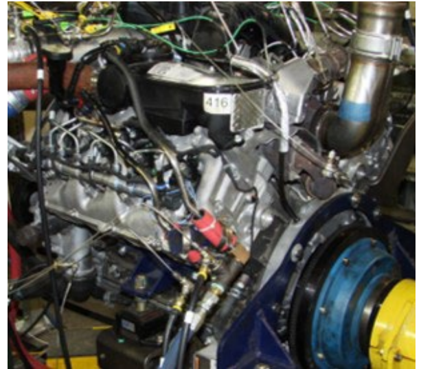
Engine Test Setup
