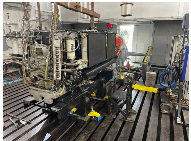
Engine Test Setup
