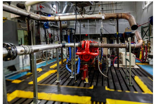
Engine Test Setup
